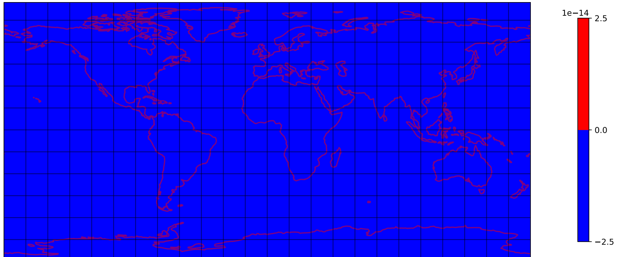
SQG psi 500 hpa 0000h - T031 expid=101
