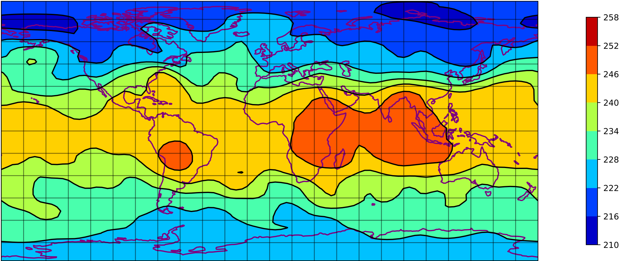
SQG t 200 hpa 0000h - T031 expid=101
