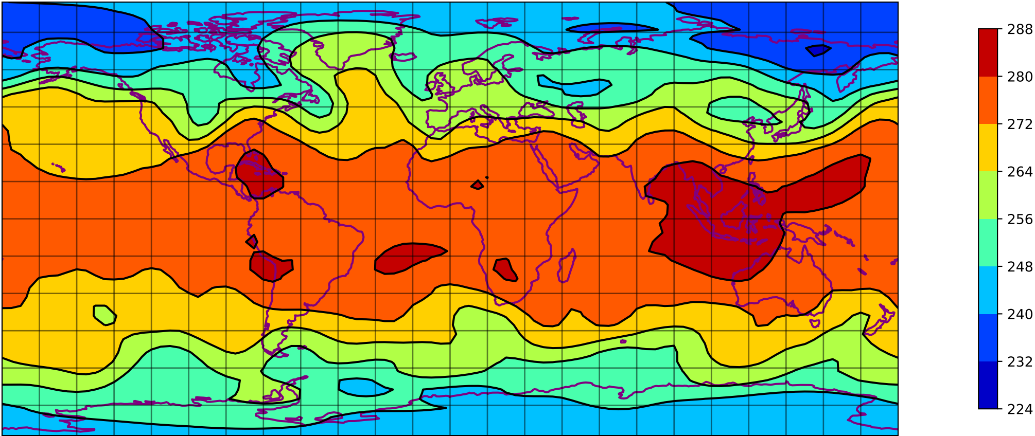
SQG t 500 hpa 0000h - T031 expid=101
