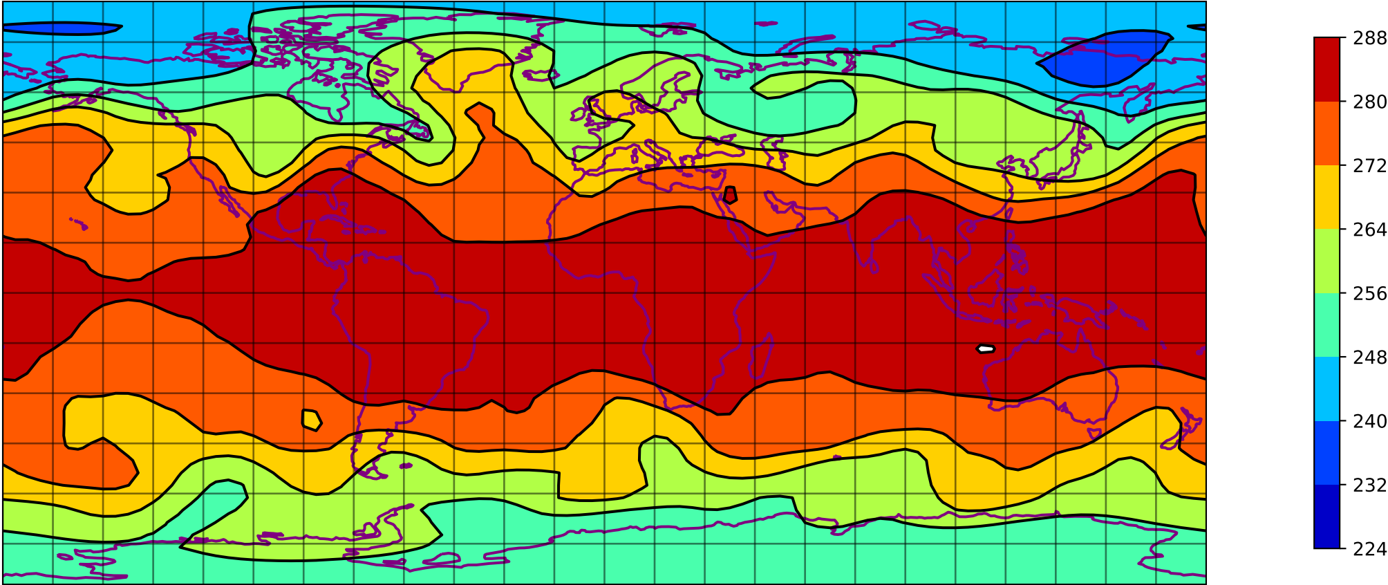
SQG t 800 hpa 0000h - T031 expid=101
