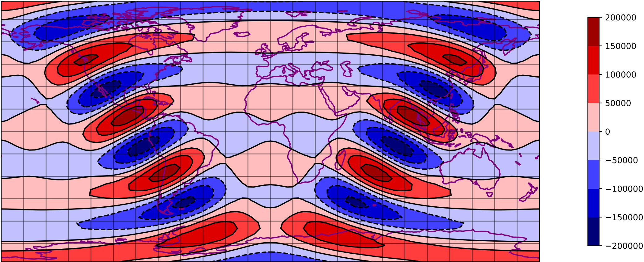
SQG u 200 hpa 0000h - T031 expid=101
