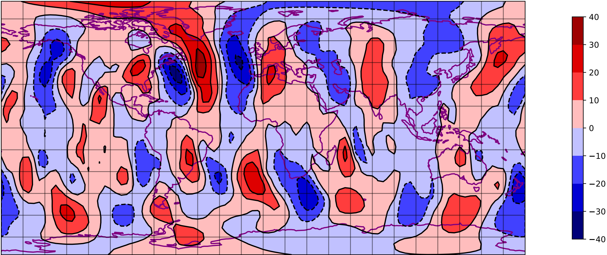
SQG v 200 hpa 0000h - T031 expid=101
