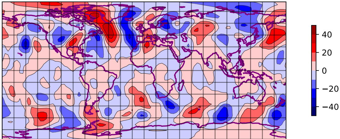
SQG v 500 hpa 0000h - T031 expid=101
