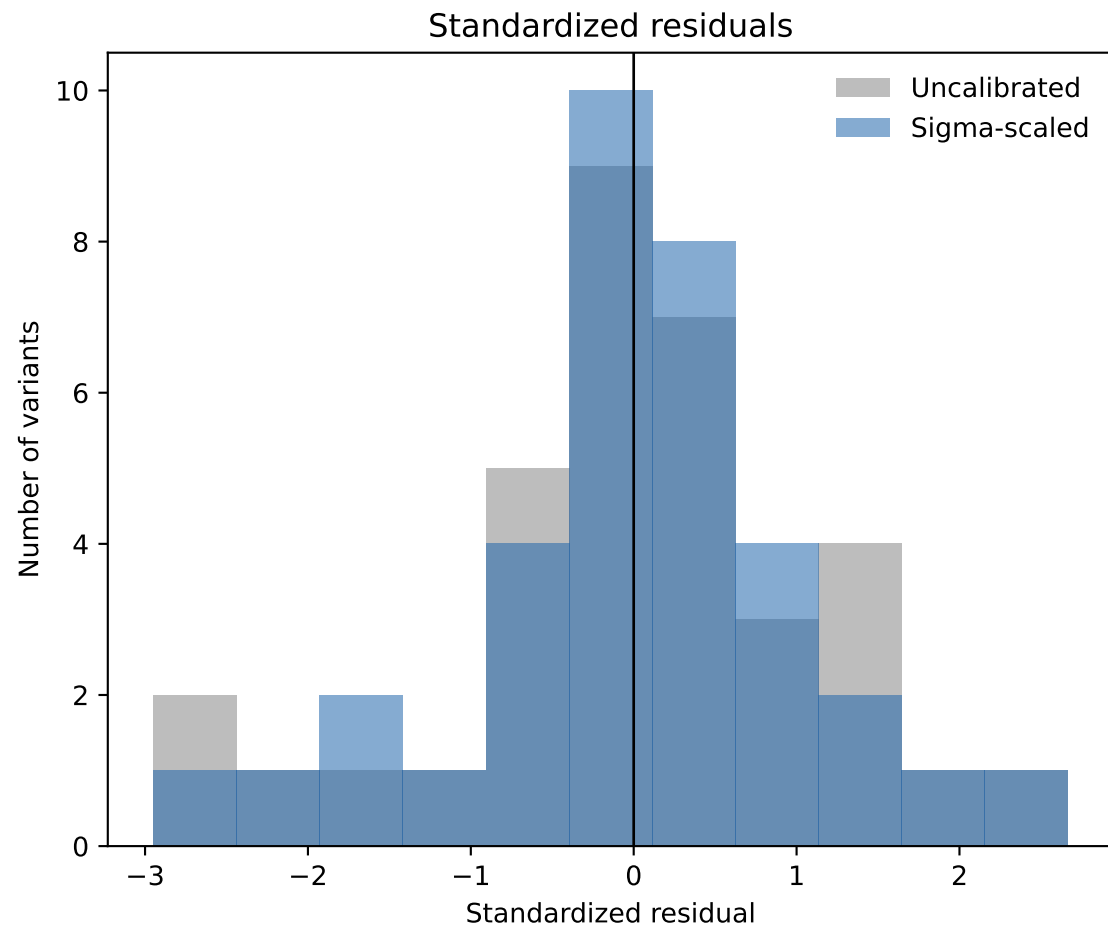
GP uncertainty before and after leakage-safe sigma scaling (deployment c=1.120)
