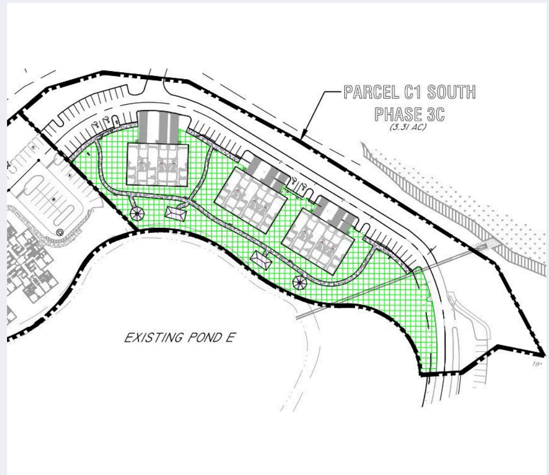
SITE PLAN · PARCEL C1 SOUTH, PHASE 3C (3.31 AC), ALONG EXISTING POND E
