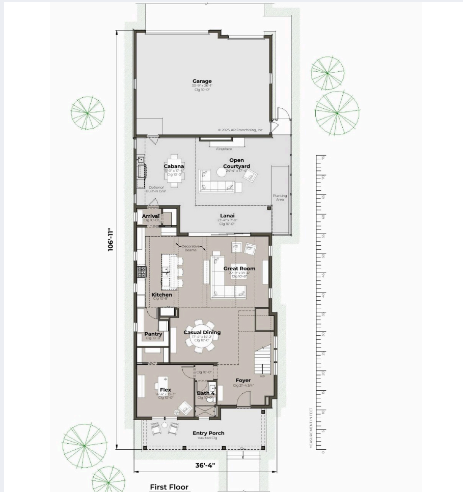
FIRST FLOOR · PLAN 1894B-OAKLAND PARK-01 · © AR FRANCHISING, INC.
