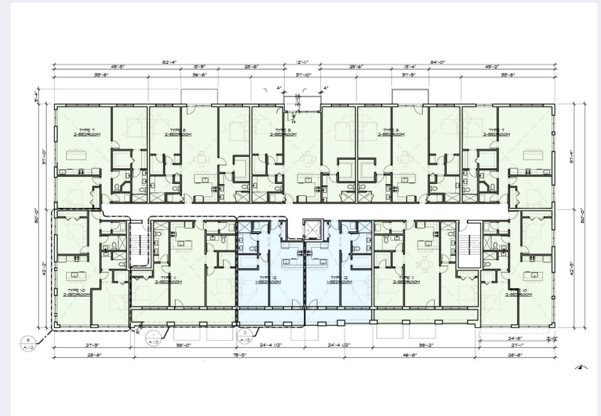
BUILDING C · FOURTH FLOOR PLAN
