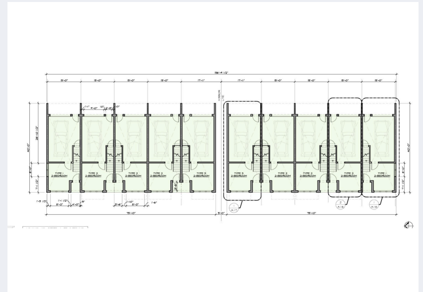
BUILDING D • FIRST FLOOR PLAN
