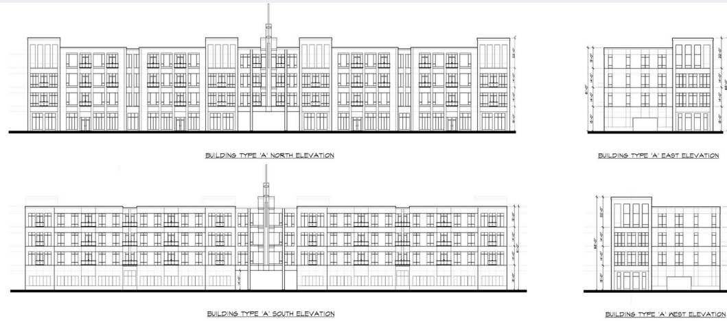
BUILDING A · NORTH, EAST, SOUTH AND WEST ELEVATIONS
