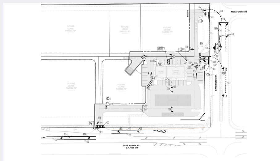
PERMITTED CONSTRUCTION PLAN • PHASE 1 LAYOUT
