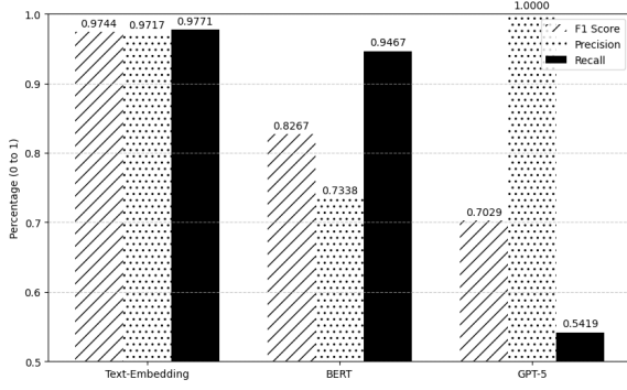
Fig. 5. F1 Score, Precision and Recall for text-embedding and BERT models on the imbalanced dataset with a 0.3 threshold. The BERT model has a significantly lower percentage in all metrics. Dropping down to 0.73 in terms of precision. We attribute this to a larger dataset in general. GPT-5 is presented here as a baseline.
