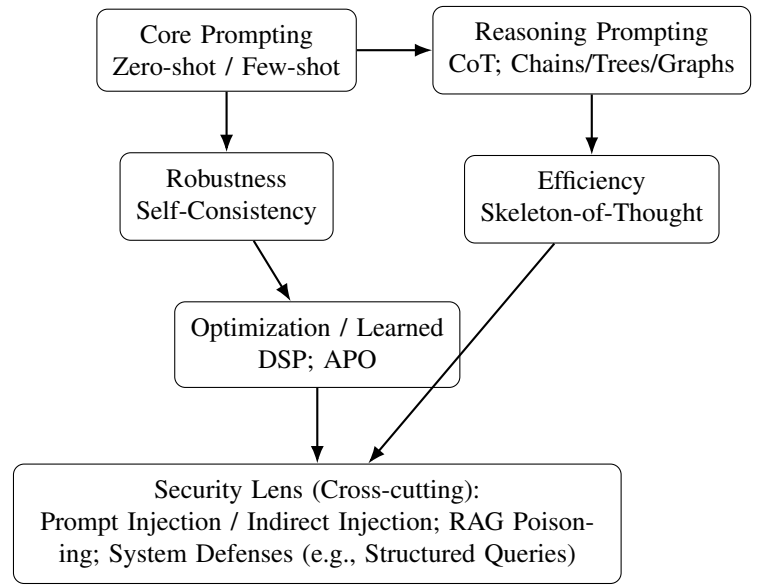
Fig. 1. Taxonomy used in this survey. The security lens is cross-cutting: it applies to all prompting and optimization families in systems that ingest untrusted content.
