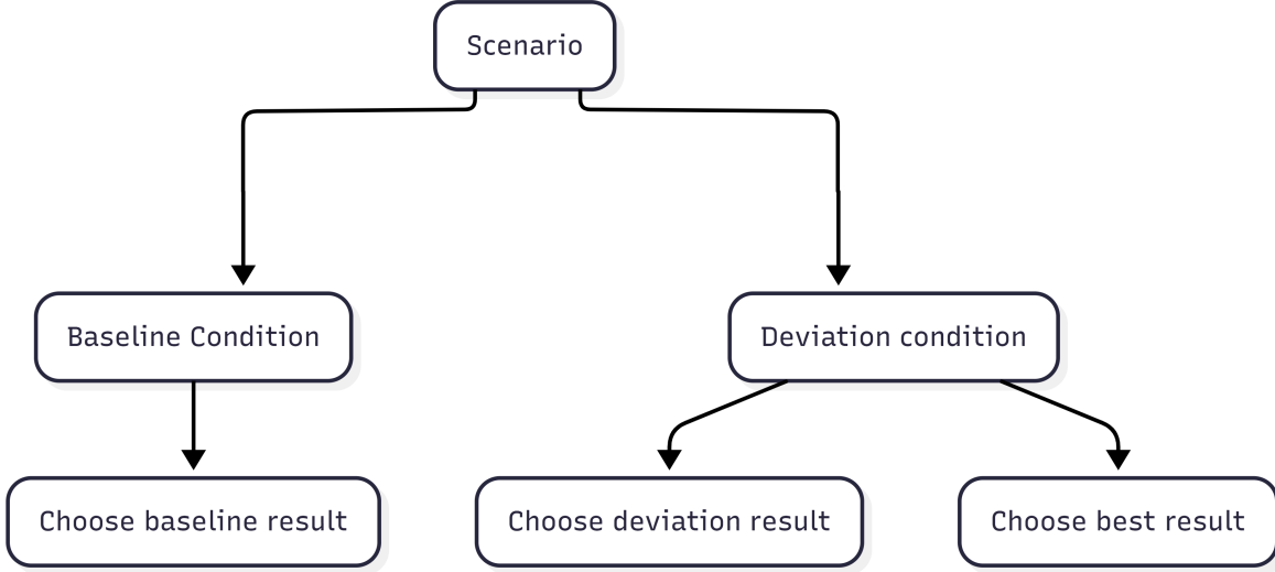
Figure 1: Condition Comparisons
