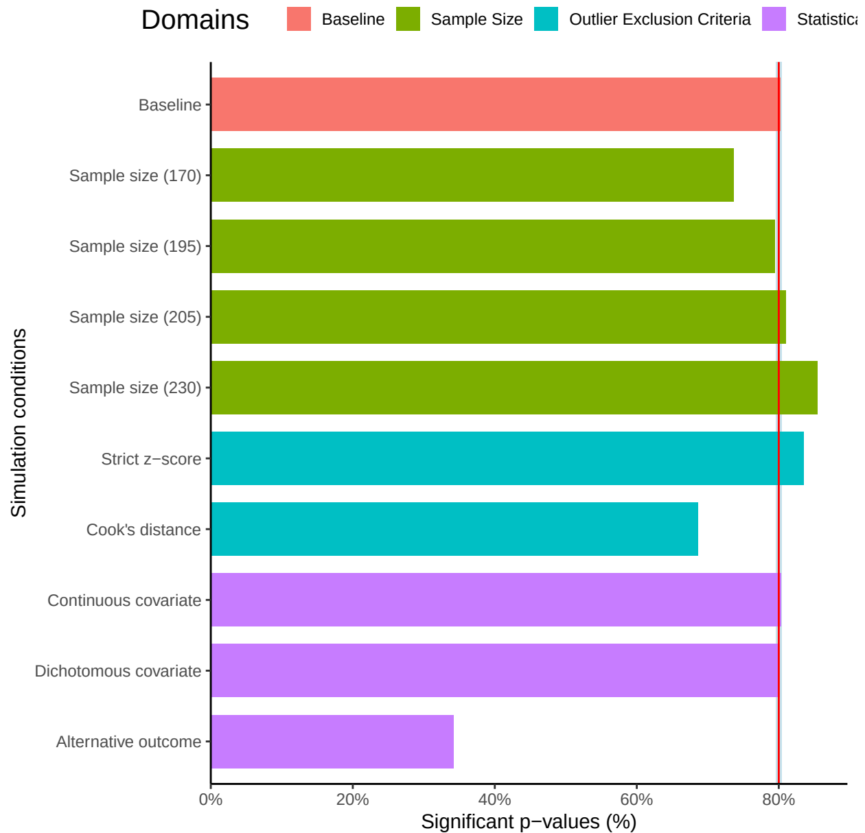
Figure B1 Robust Power per Condition
