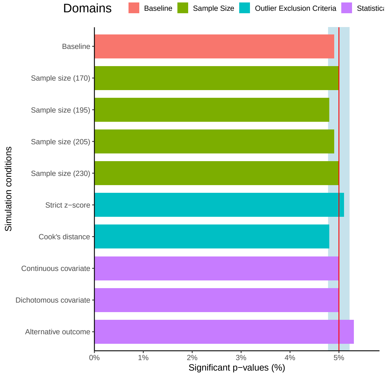
Figure B2 Robust Type I Error per Condition
