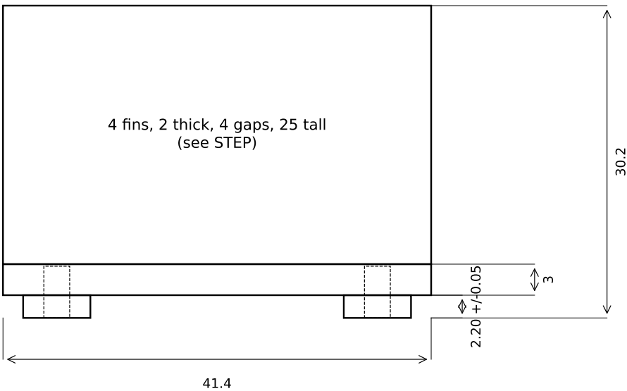
SIDE VIEW (fins up; feet sit on the board)
