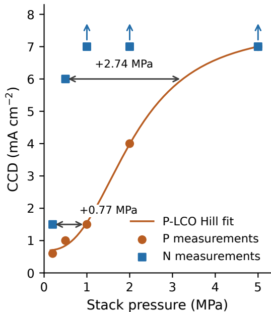
(a) Measured CCD and pressure equivalence
