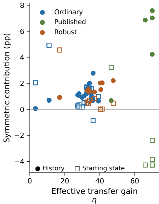
(a) History and starting-state contributions
