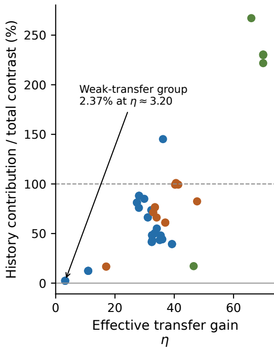
(b) The allocation is not identified
