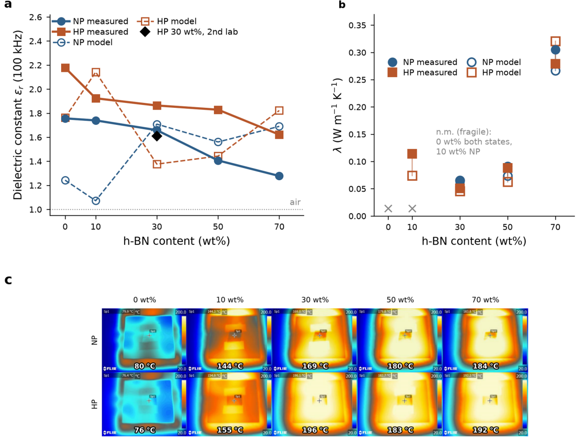
Figure 2: Measured dielectric and thermal properties of PI/h-BN films ( n = 1 per condition). (a) Dielectric constant at 100 kHz vs. h-BN content for NP and HP films; filled symbols, measured; open symbols joined by dashed lines, three-phase LN predictions at each film’s measured open porosity; black diamond, independent measurement of the HP 30 wt% film (KOPTRI, ASTM D150), not used in fitting. (b) Thermal conductivity vs. h-BN content; open symbols, single-parameter LN predictions ( \lambda_{\text{BN,eff}} fitted; A = 5.5 , \phi_{\text{max}} = 0.60 fixed), joined to the measured value by a tie-line; crosses mark compositions that could not be measured (film fragility). (c) Infrared thermography of all ten films on a 200 °C stage after [X] min equilibration; annotated values are uncorrected radiometric spot temperatures and are comparative, not absolute. Parity plot and porosity-sensitivity curves are given in Figures S2 and S3.
