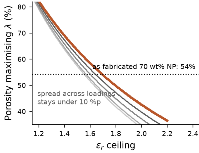
Figure S5: Porosity that maximizes \lambda under each \varepsilon_r ceiling for 0–70 wt% h-BN (light to dark grey, 0–50 wt%; orange, 70 wt%). The dotted line marks the as-fabricated porosity of the 70 wt% NP film (54%).
