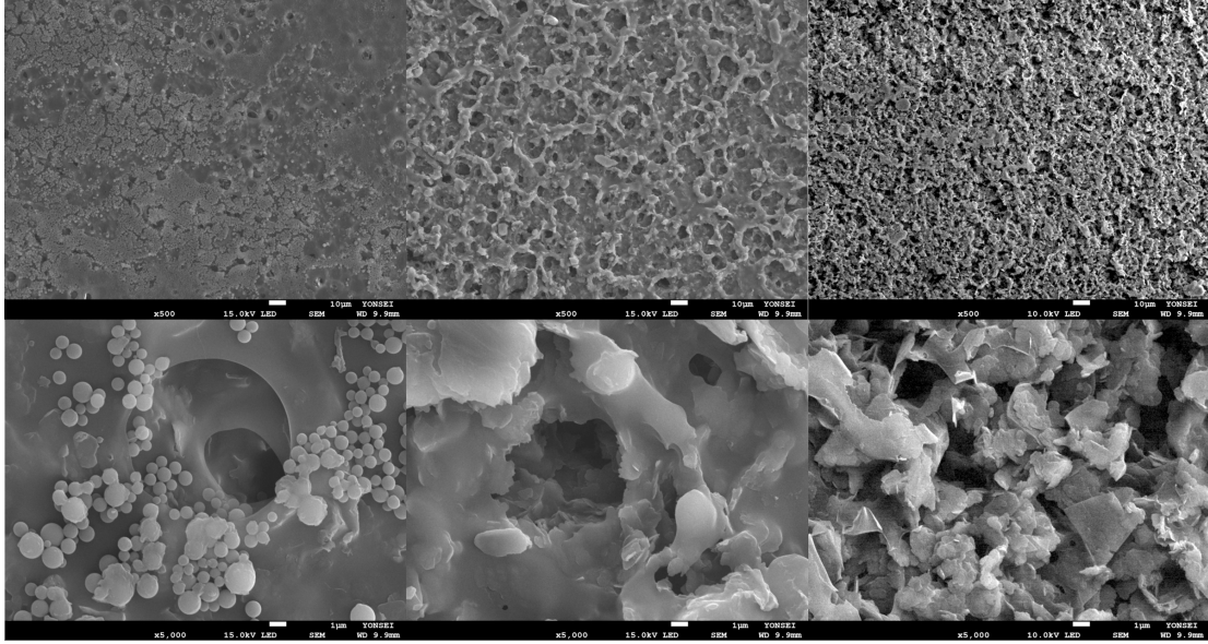
Figure S7: Top-view FE-SEM micrographs of PI/h-BN films at 30, 50, and 70 wt% h-BN (columns) at two magnifications (rows). Label the rows by magnification ( \times 500 , \times 5,000 ) and the columns by composition on the figure.
