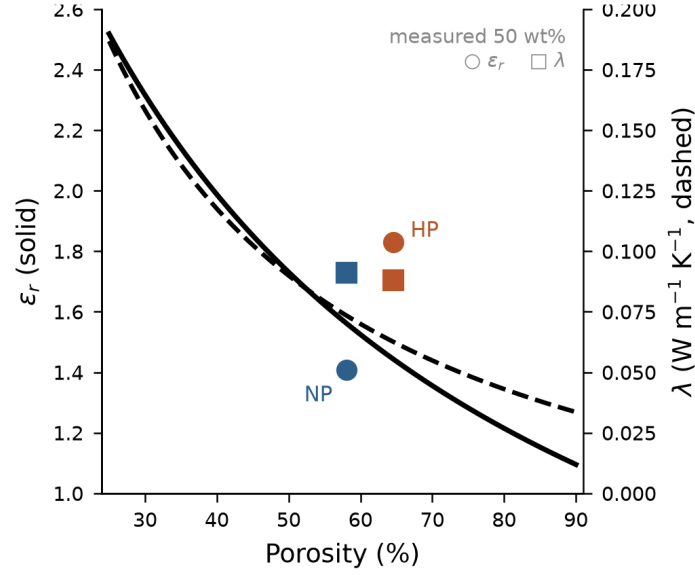
Figure S3: Porosity sensitivity at fixed 50 wt% h-BN: \varepsilon_r (left axis, solid) and \lambda (right axis, dashed) from the calibrated three-phase LN model. Circles and squares mark the measured NP and HP 50 wt% films ( \varepsilon_r and \lambda , respectively).
