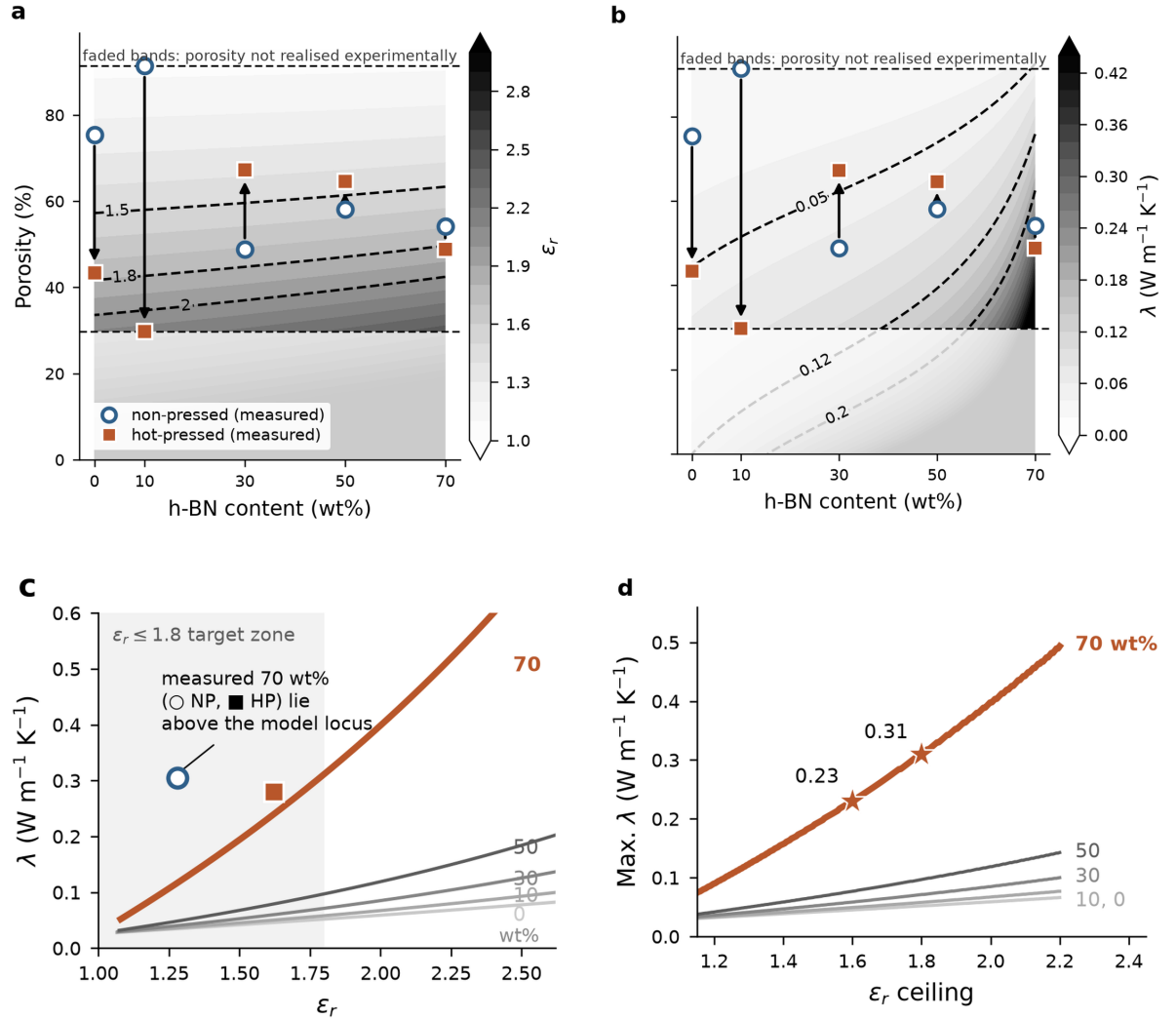
Figure 4: Design maps Model-guided design (3-phase three-phase LN model, calibration of Table 1) for. (a, b) dielectric constant \epsilon_r and (b) thermal conductivity \lambda ( \text{W/mK} ) as functions of vs. h-BN content and porosity. Measured: measured NP (open circles) and HP (filled squares) states are overlaid; arrows indicate indicating the NP→HP processing trajectory. The faded bands above 91% and below 30% porosity lie outside the range realised by any of film. (c) \epsilon_r - \lambda loci for each loading with porosity swept along each curve; the measured 70 wt% films lie above their own locus. (d) Maximum \lambda attainable under a given \epsilon_r ceiling with porosity optimized at each point; stars mark the map there is extrapolation rather than interpolation between measured states \epsilon_r \leq 1.6 and \epsilon_r \leq 1.8 operating points at 70 wt%. The absolute levels of panels (a)-(d) inherit the dielectric uncertainty quantified in Section 4.2. Feasible-window and porosity-optimum panels are given in Figures S4 and S5.
