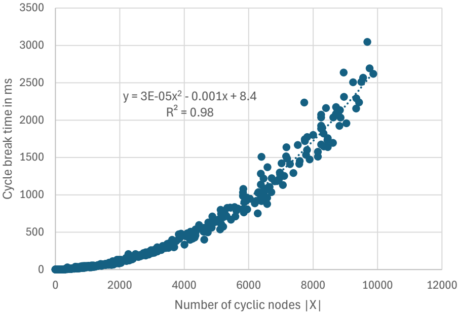
Cycle break time - prototype implementation
