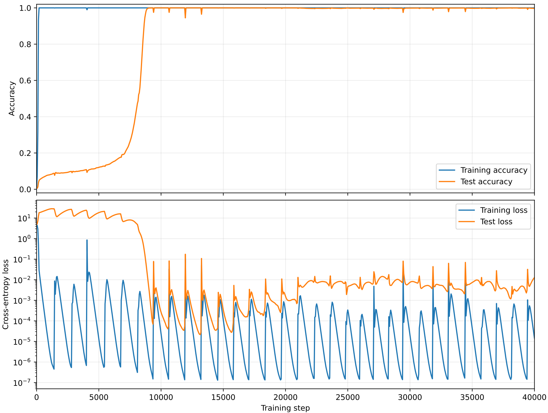
Modular-addition training trajectory modular-addition-training-s1-5f1bc9dee7ab
