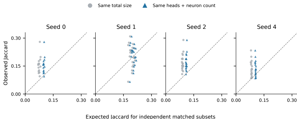
Figure S1: Small raw overlaps exceed the matched random-subset expectation in aggregate. The 78 final within-family pairs, separated by model. Each pair is plotted against its exact expected Jaccard under two matching rules. Points above the diagonal overlap more than their matched expectation. Seed 1 lies closer to equality than the other models. The two marks for a pair share the same observed value; they are alternative baselines, not additional observations.
