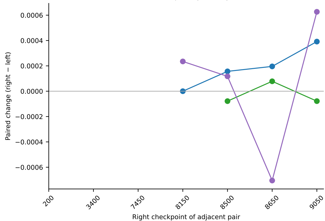
Matched-sparsity fidelity \Delta
