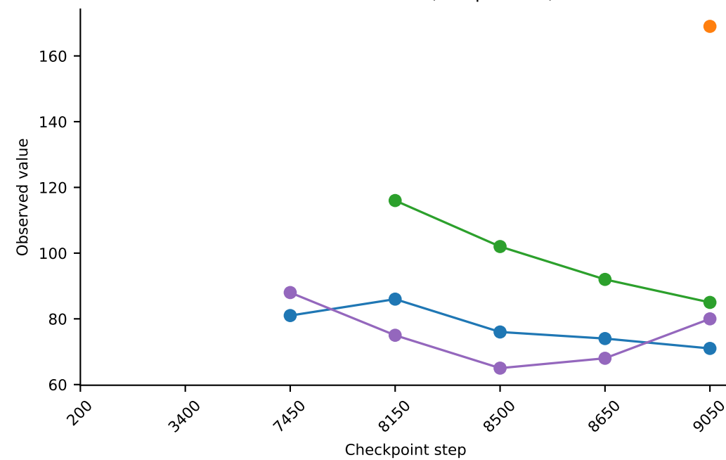
Median circuit size (components)
