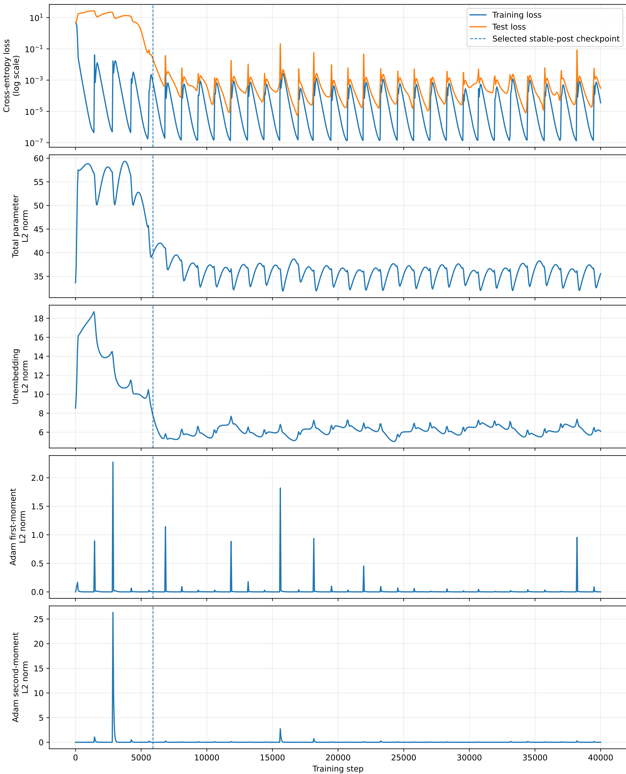
Seed-0 loss and norm diagnostics modular-addition-training-s0-5f1bc9dee7ab
