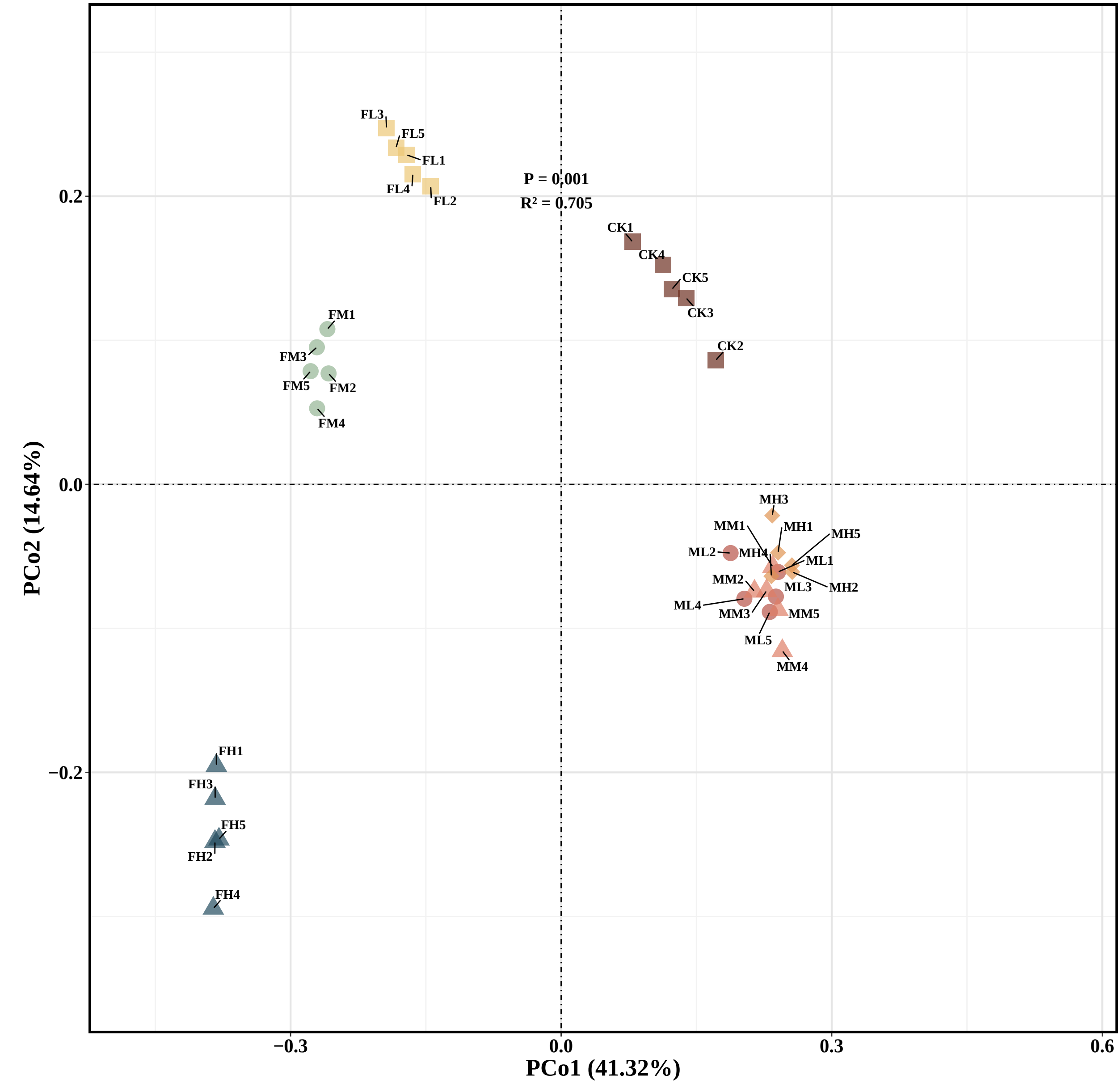
PCoA
