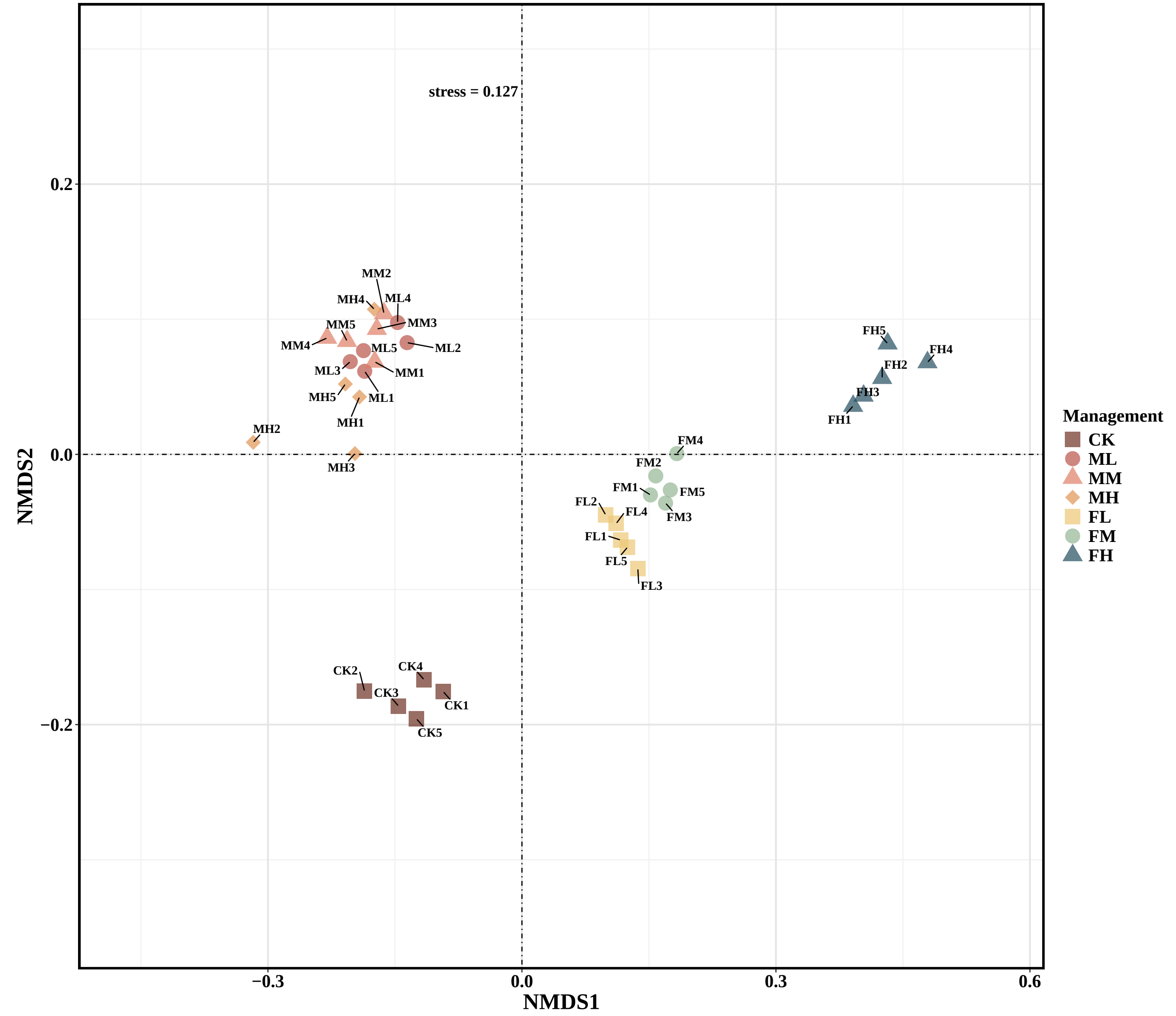
NMDS
