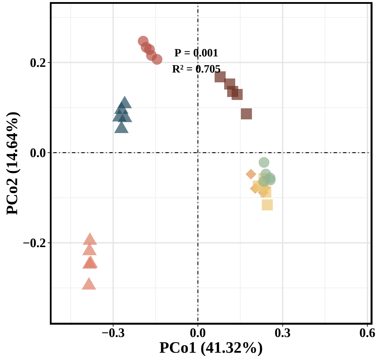
PCoA
