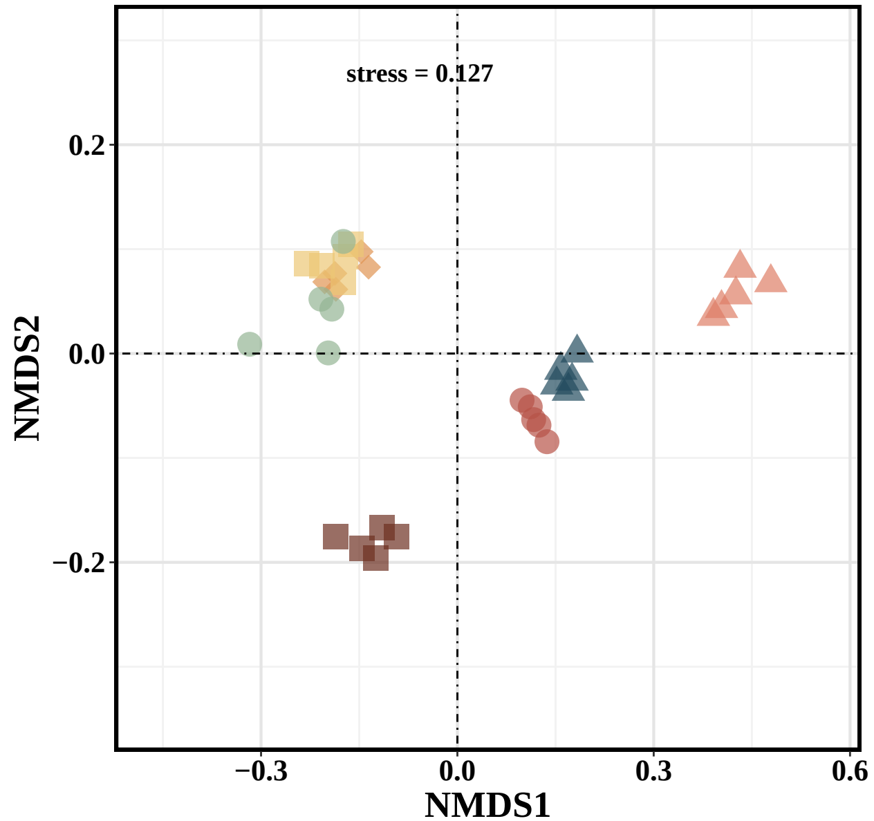
NMDS
