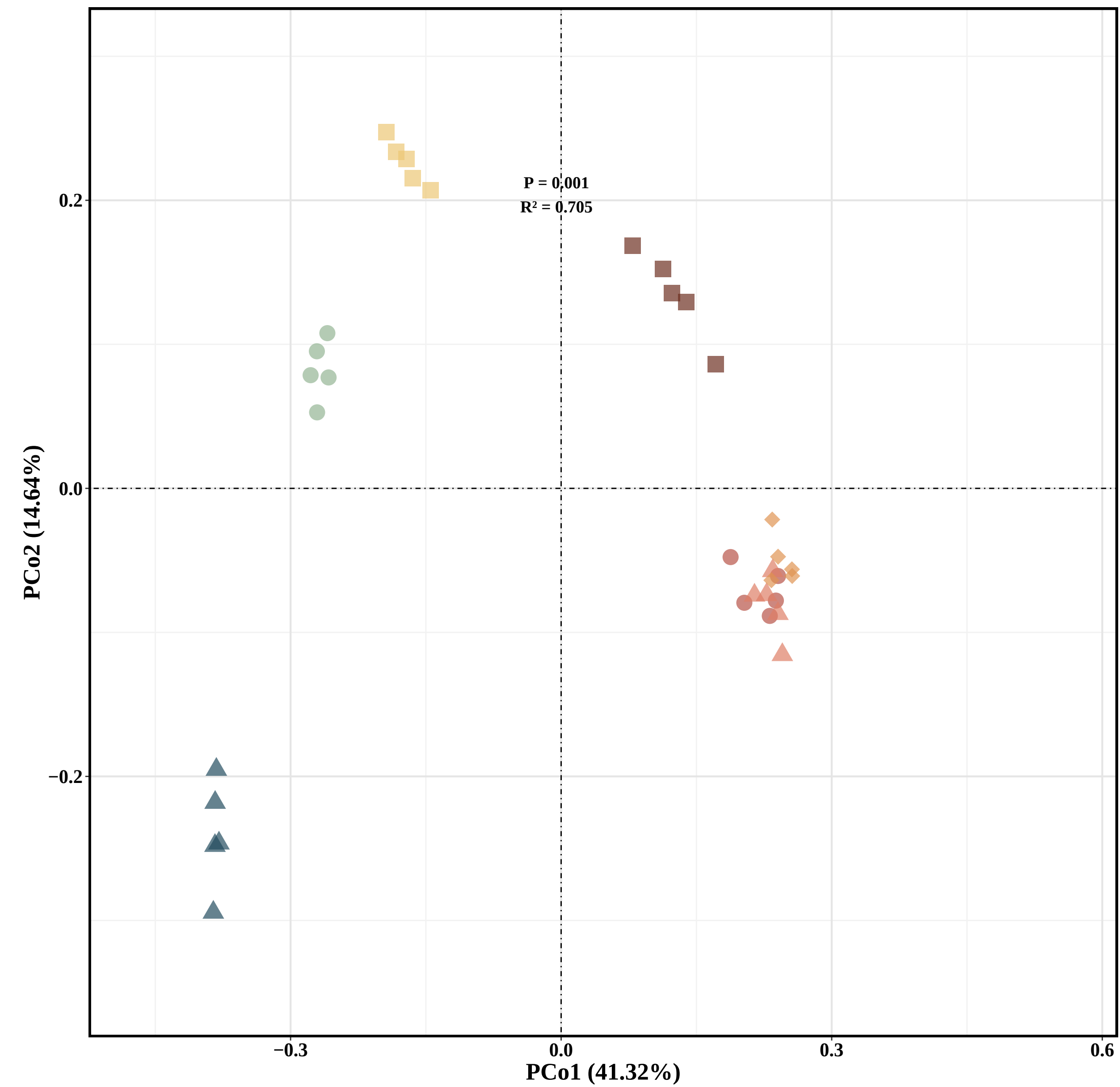
PCoA
