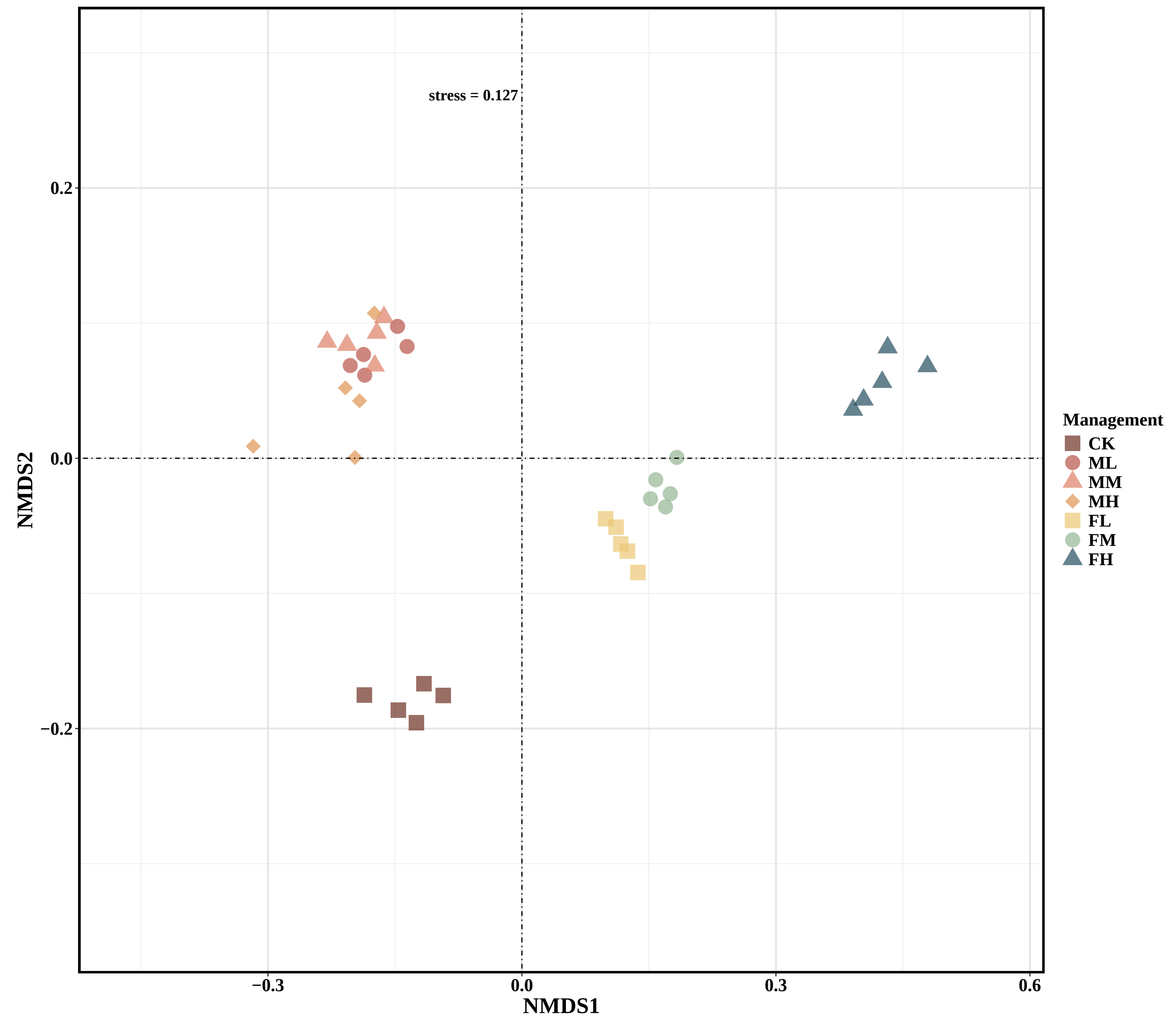
NMDS
