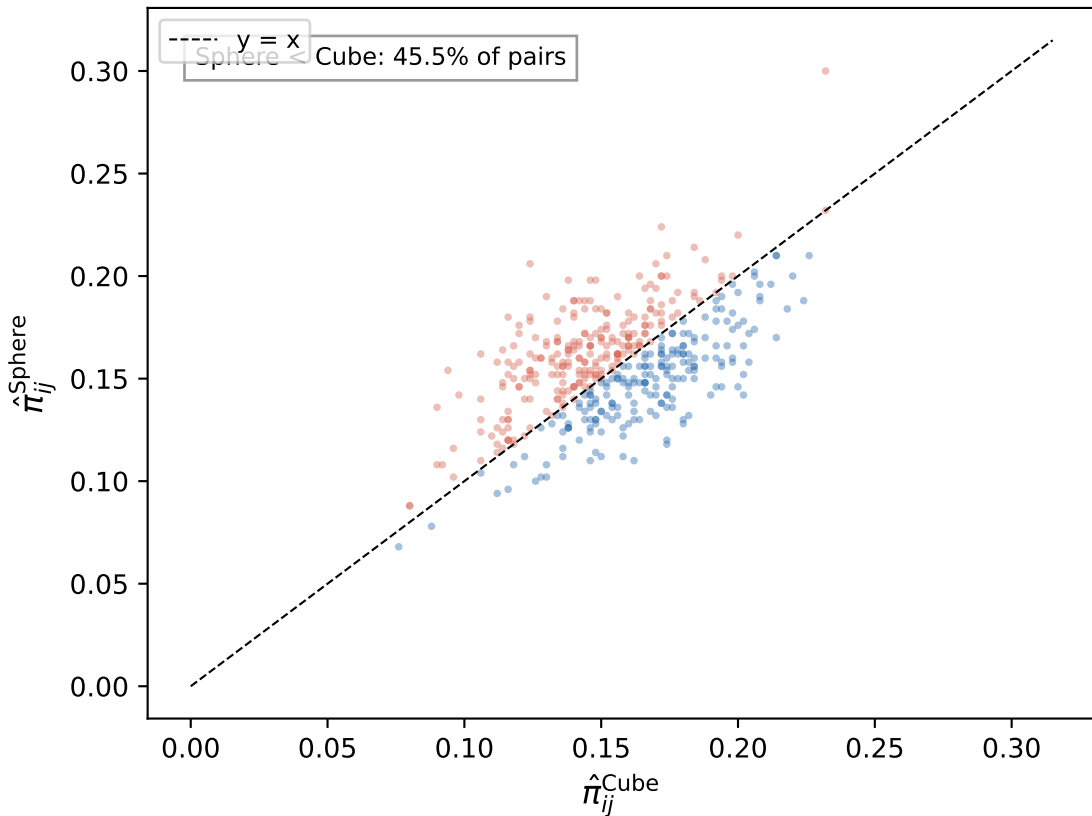
Q1 — Pairwise \hat{\pi}_{ij} compared N=30, p=5, f=0.4, correlated, alpha=0.2
