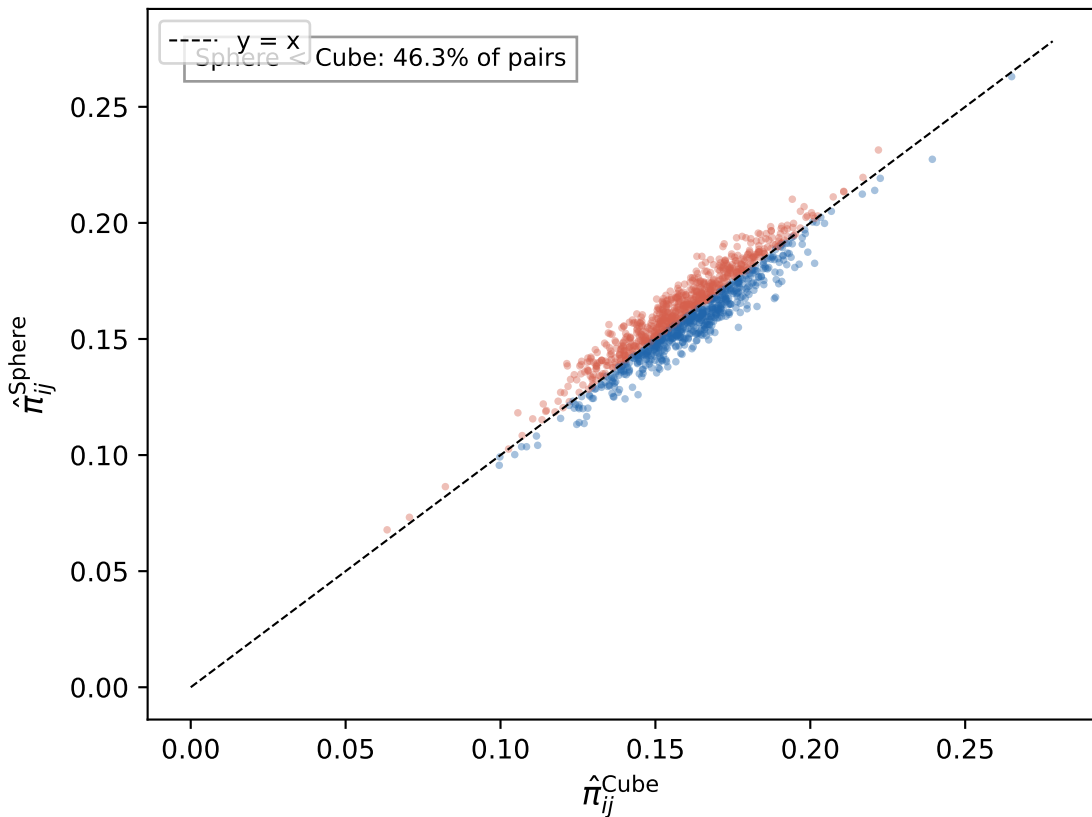
Q1 — Pairwise \hat{\pi}_{ij} compared N=50, p=10, f=0.4, correlated, alpha=0.2
