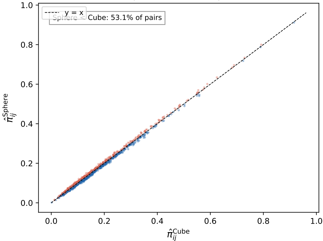
Q1 — Pairwise \hat{\pi}_{ij} compared N=50, p=2, f=0.4, mixed, alpha=0.2
