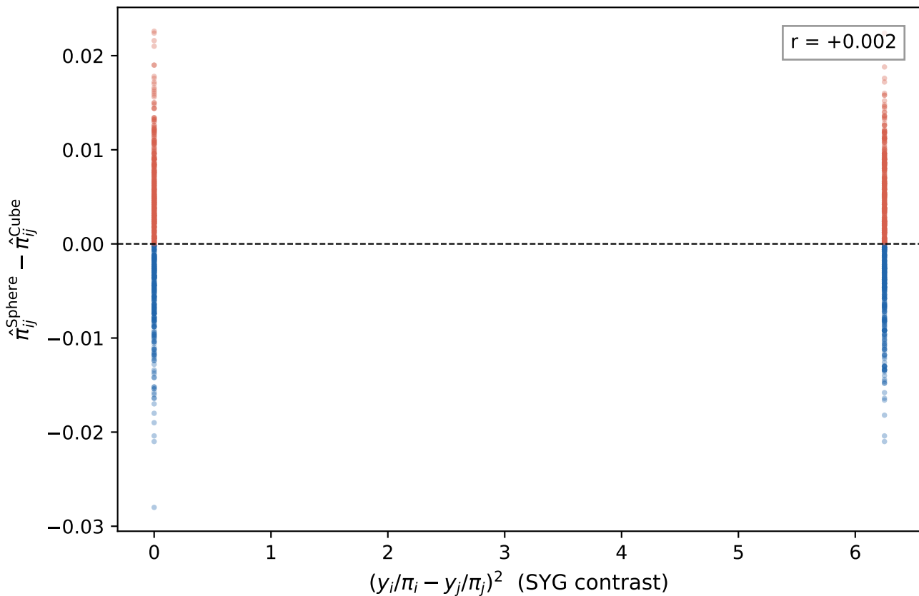
Q2 — Is the inequality concentrated on large contrasts? N=50, p=2, f=0.4, mixed, alpha=0.2
