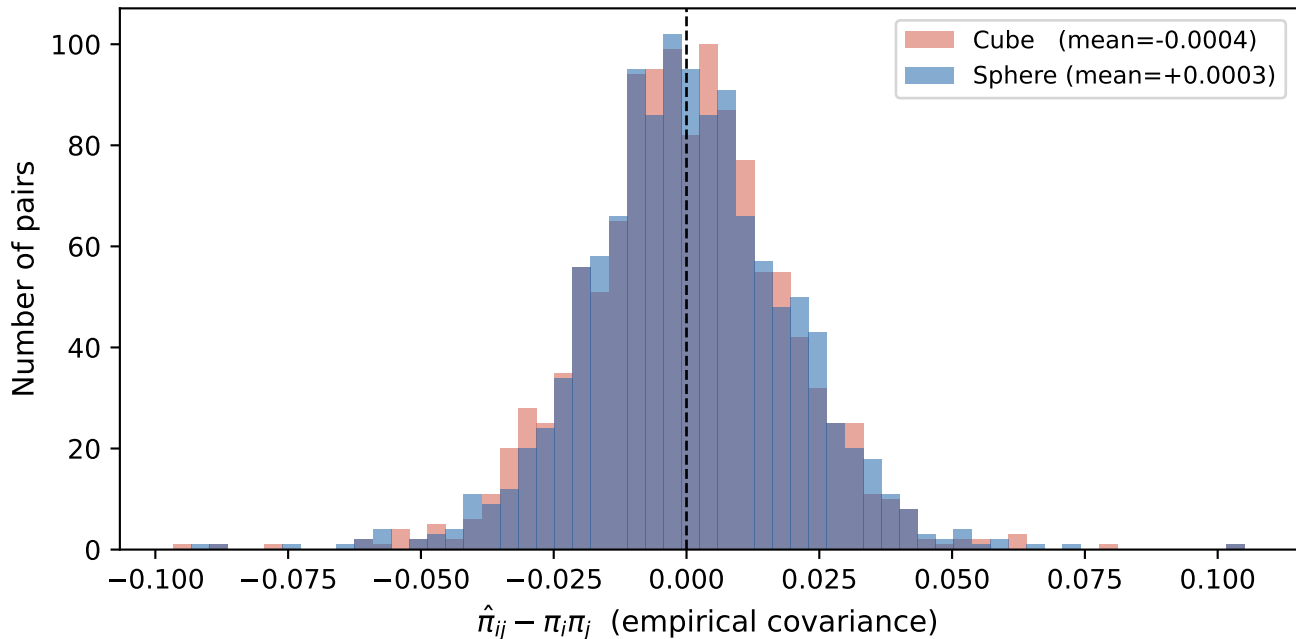
Q3 — Induced correlations vs independence N=50, p=10, f=0.4, correlated, alpha=0.2
