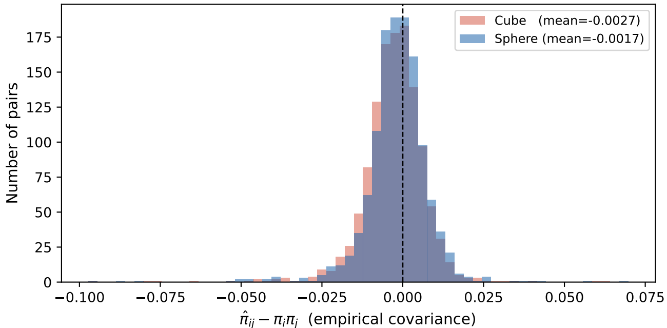
Q3 — Induced correlations vs independence N=50, p=2, f=0.4, mixed, alpha=0.2
