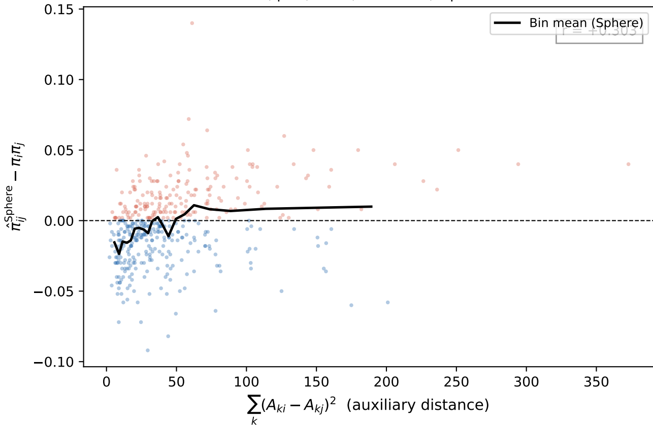
Q4 — Does auxiliary distance predict co-selection? N=30, p=5, f=0.4, correlated, alpha=0.2
