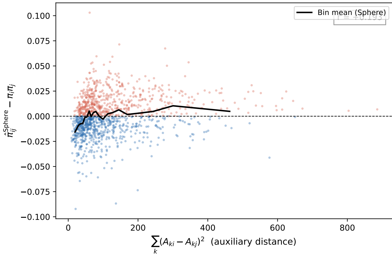
Q4 — Does auxiliary distance predict co-selection? N=50, p=10, f=0.4, correlated, alpha=0.2
