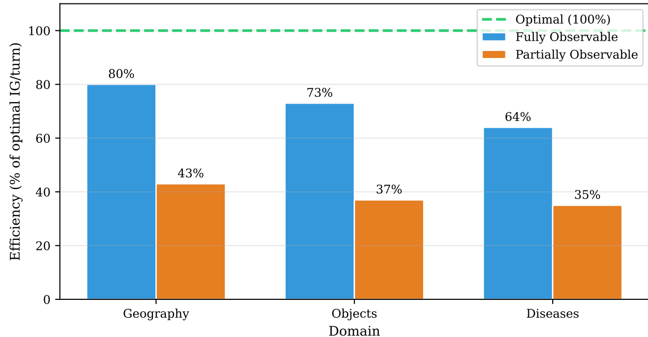
Information Gathering Efficiency vs. Theoretical Optimal
