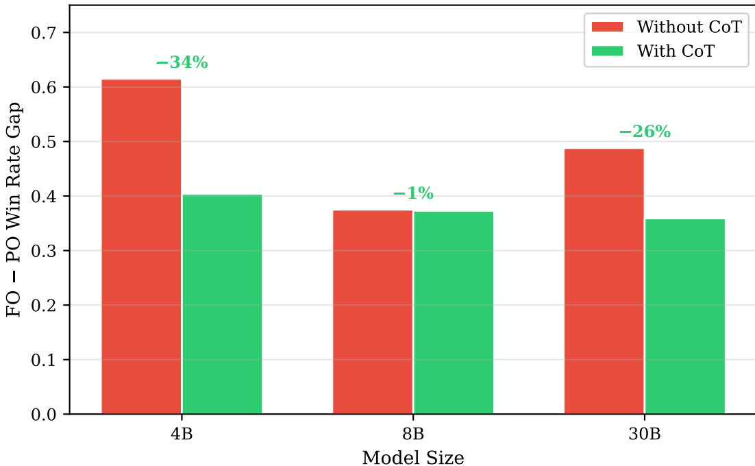
CoT Reduces the Observability Gap
