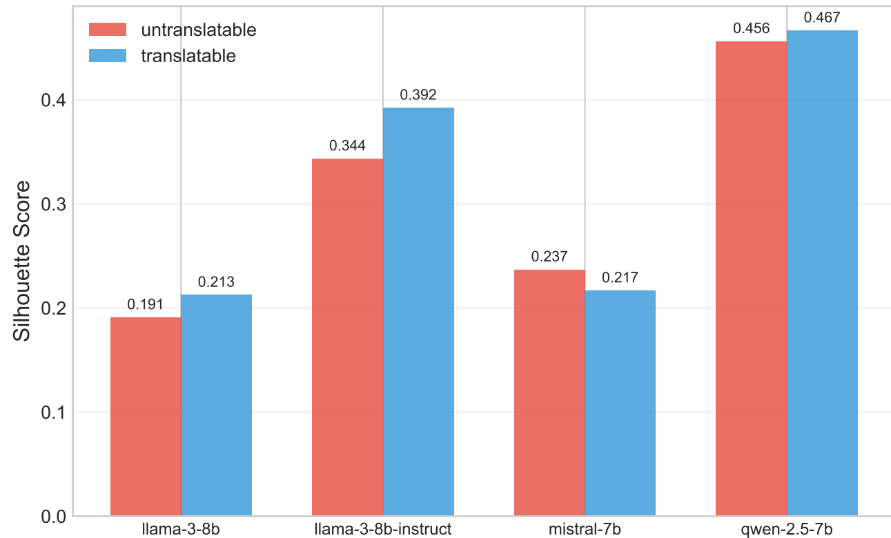
Silhouette Scores: All Models
