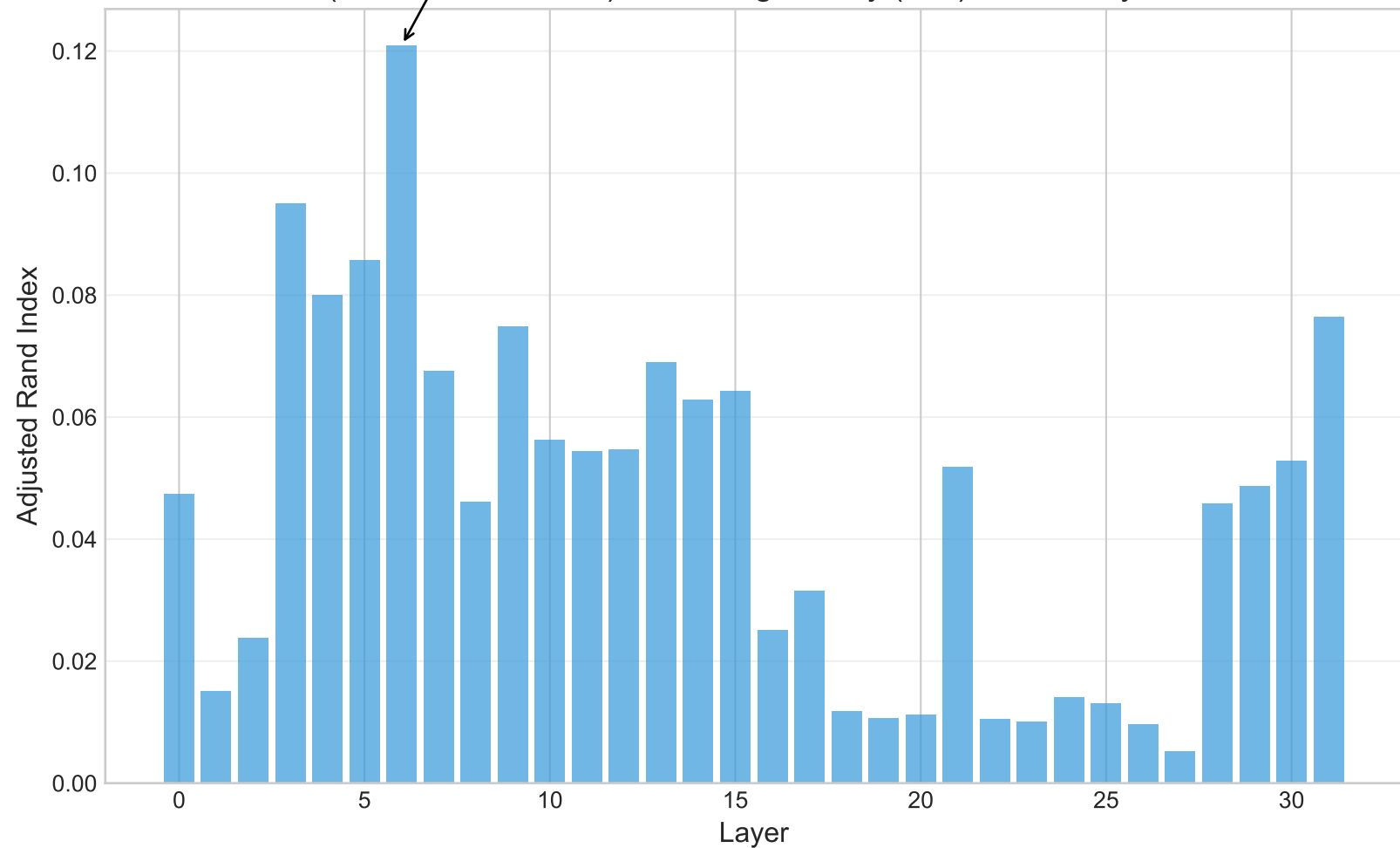
(llama-3-8b-instruct) Clustering Quality (ARI) Across Layers
