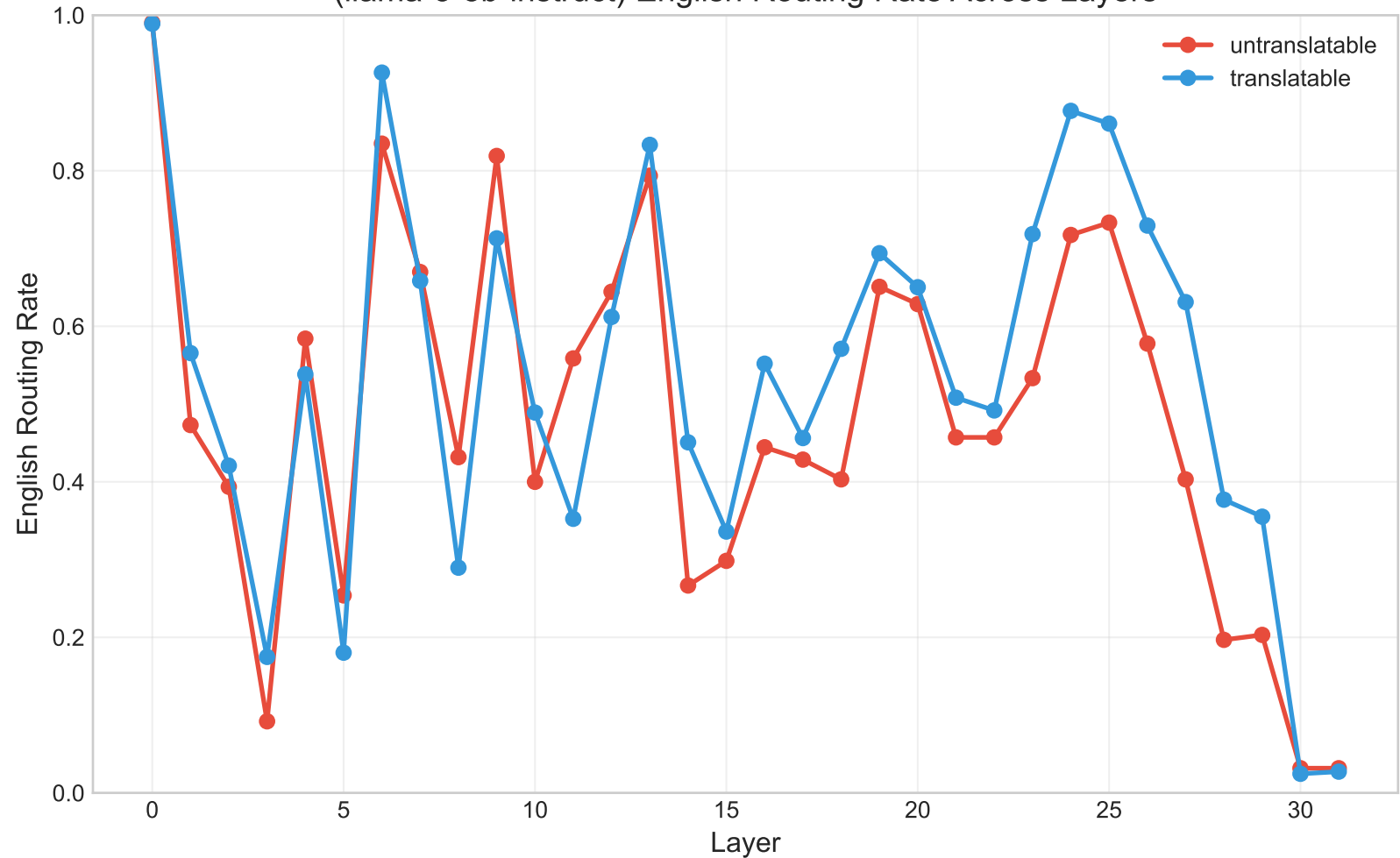
(llama-3-8b-instruct) English Routing Rate Across Layers
