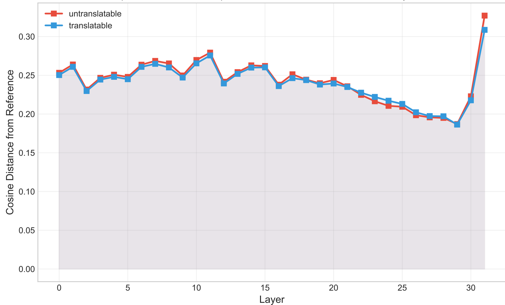
(llama-3-8b-instruct) Distance from Centroid Across Layers
