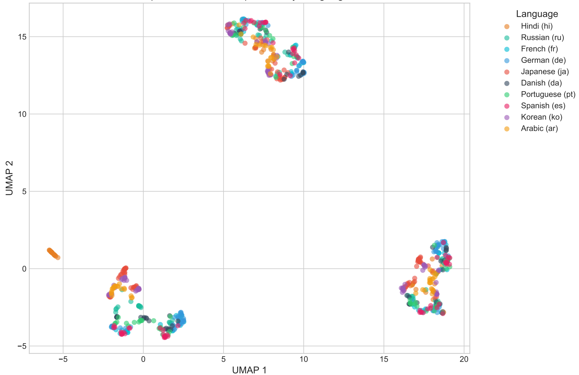
(llama-3-8b-instruct) UMAP by Language
