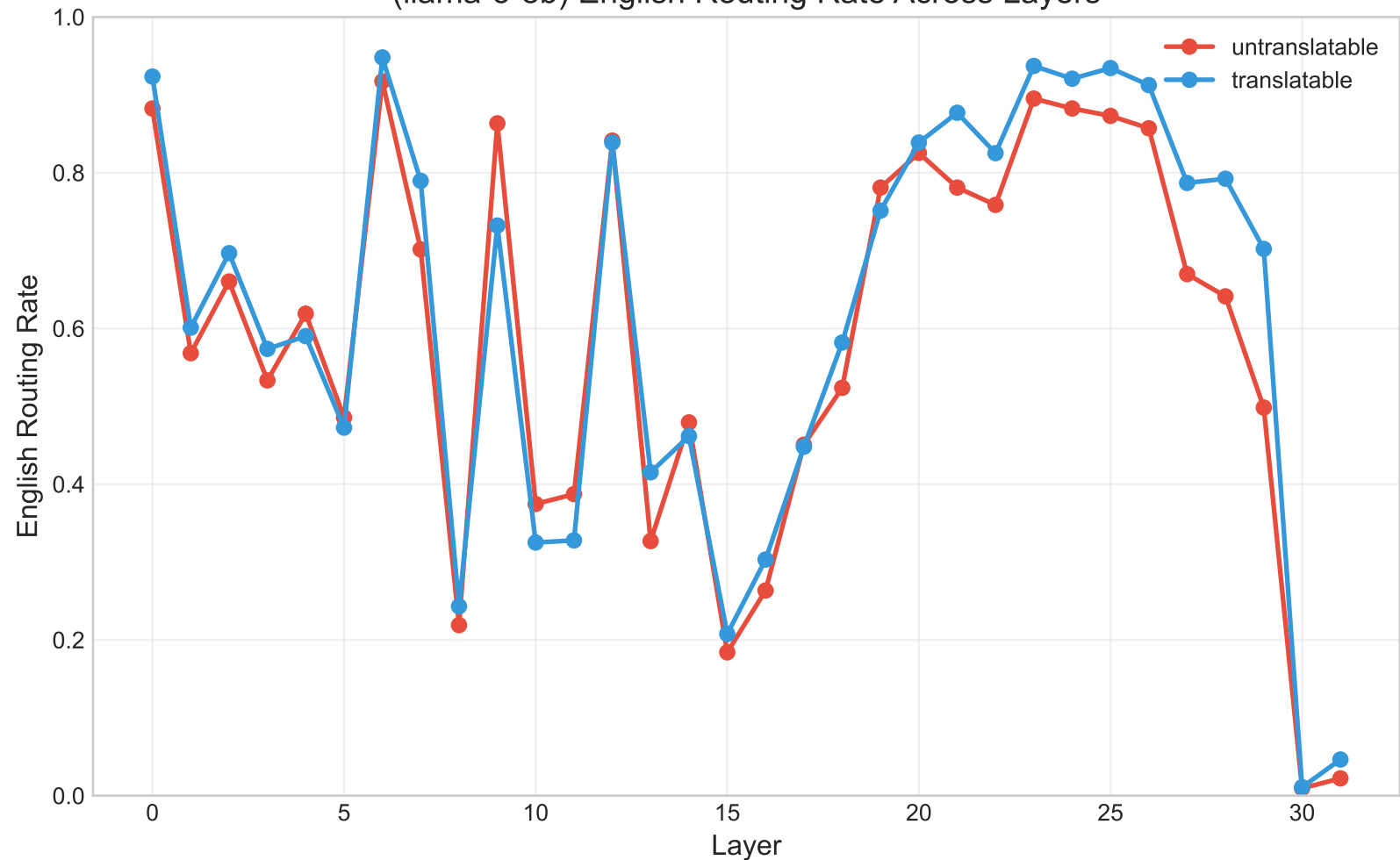
(llama-3-8b) English Routing Rate Across Layers
