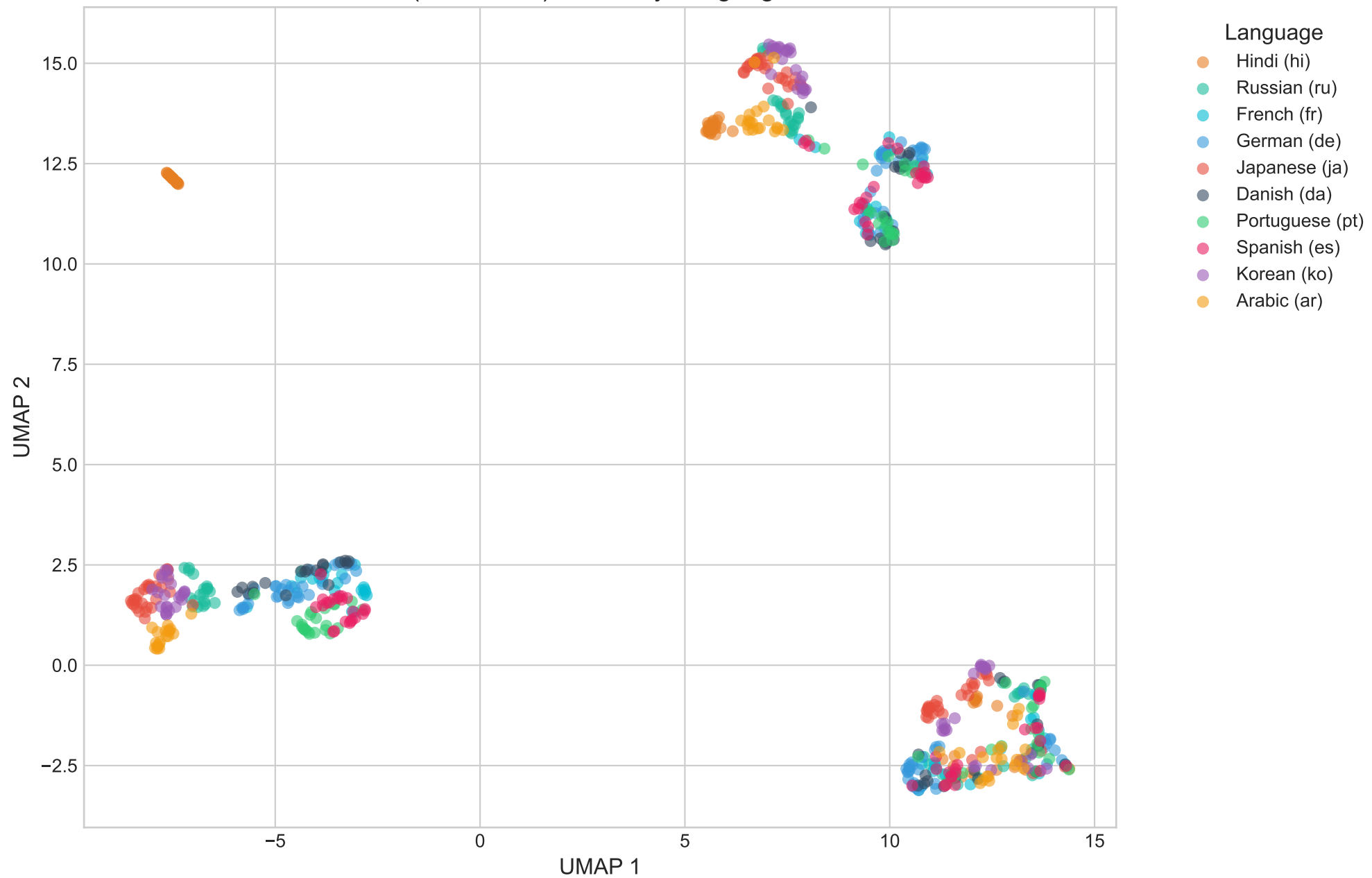
(llama-3-8b) UMAP by Language
