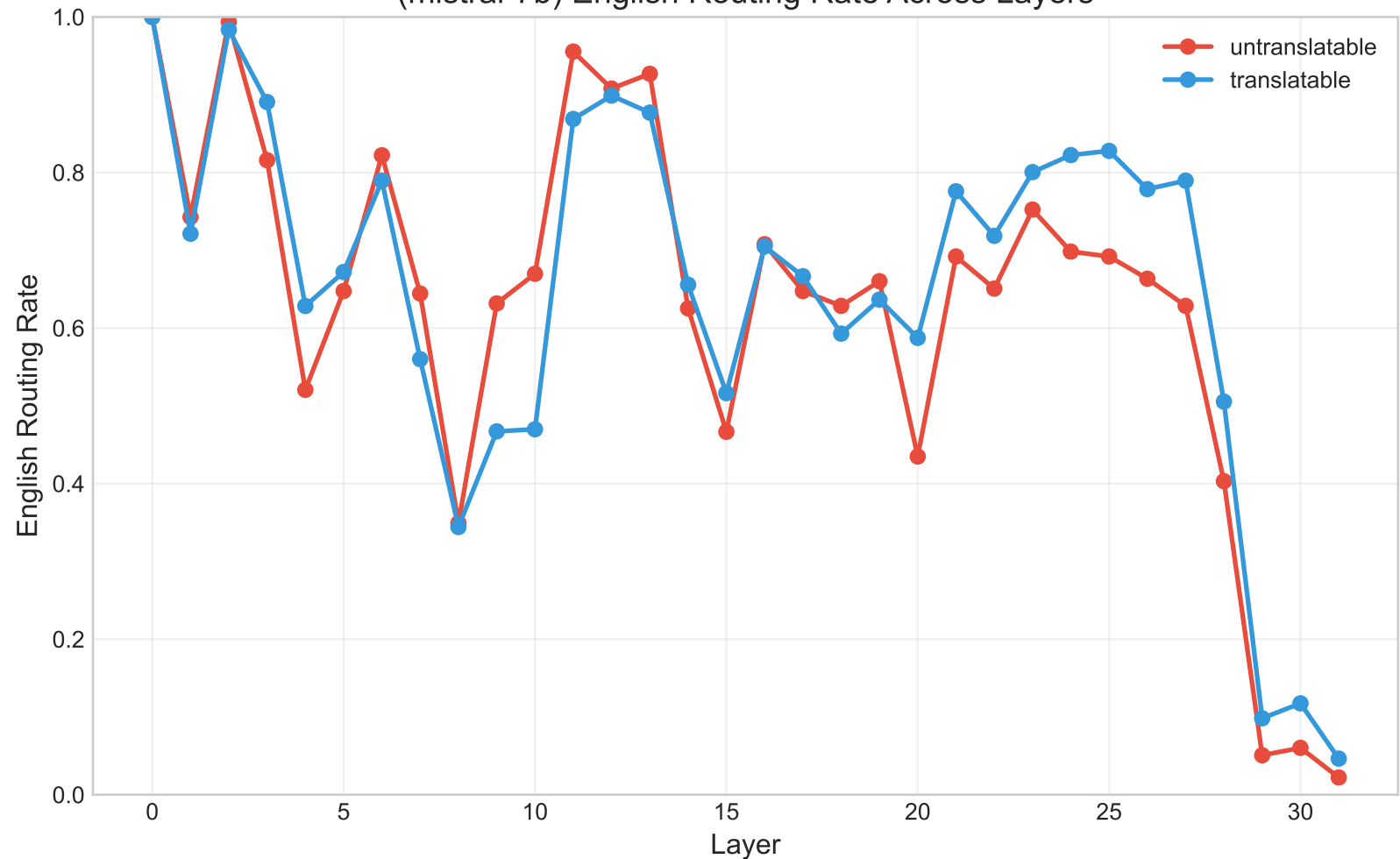
(mistral-7b) English Routing Rate Across Layers
