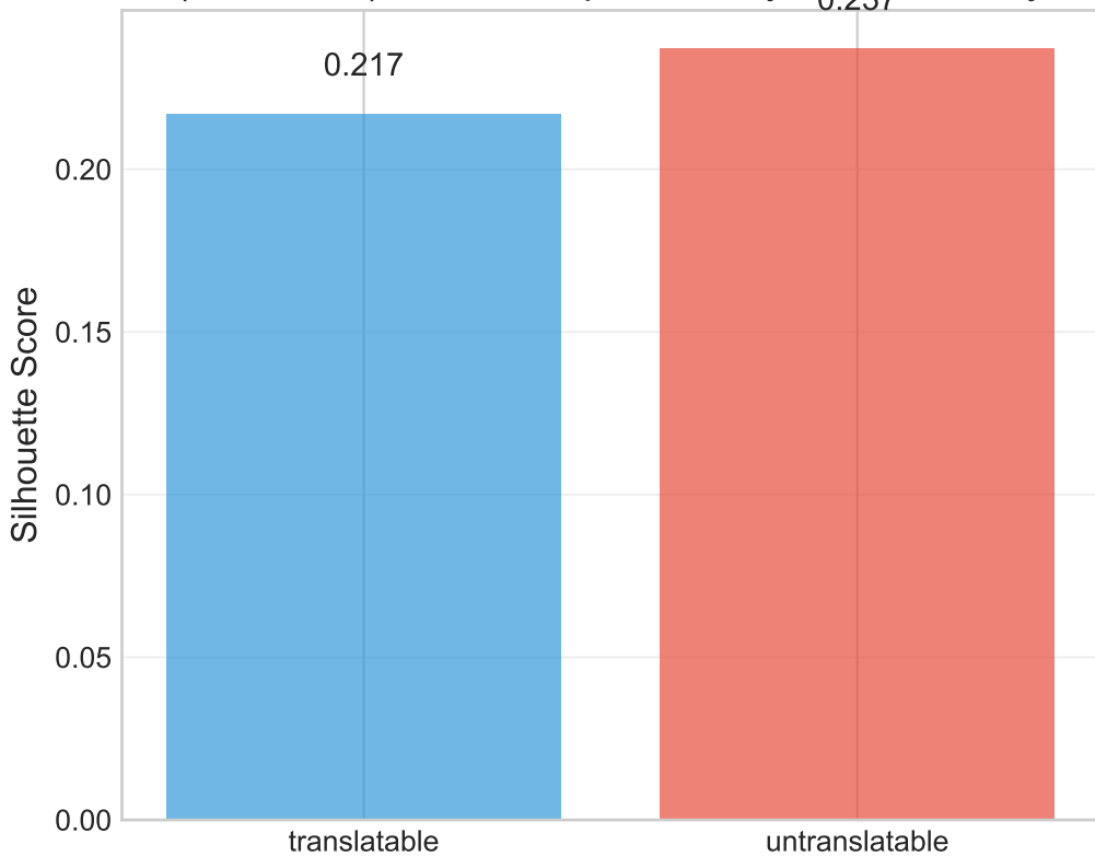
(mistral-7b) Cluster Separation by Translatability
